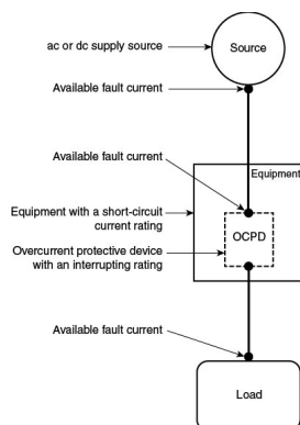
Figure 100.0 Available Fault Current.
