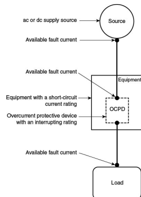
Figure 100.0 Available Fault Current.
