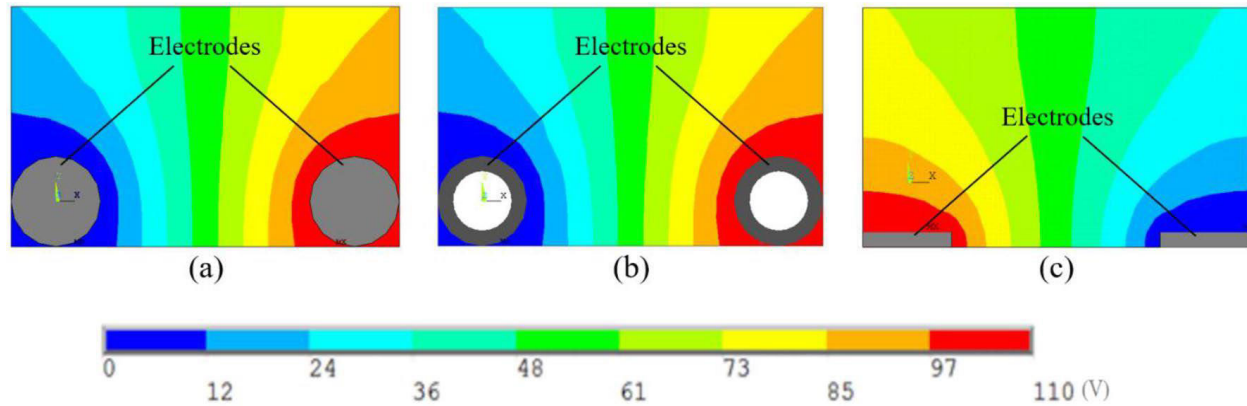
Figure 24. Voltage lines developed by different electrodes: (a) smooth solid circular bar, (b) hollow circular bar, and (c) flat bar
