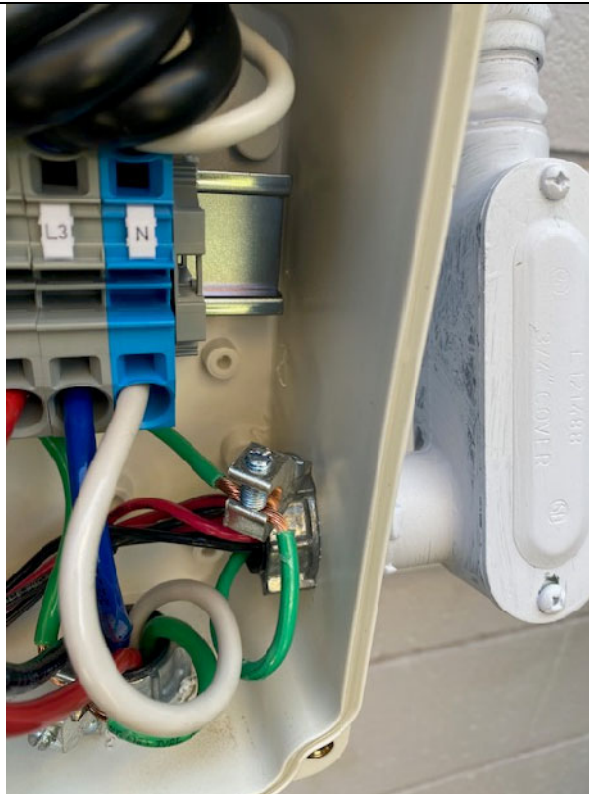
Photo 2 – Proper Bonding Completed but Not Clearly Required
