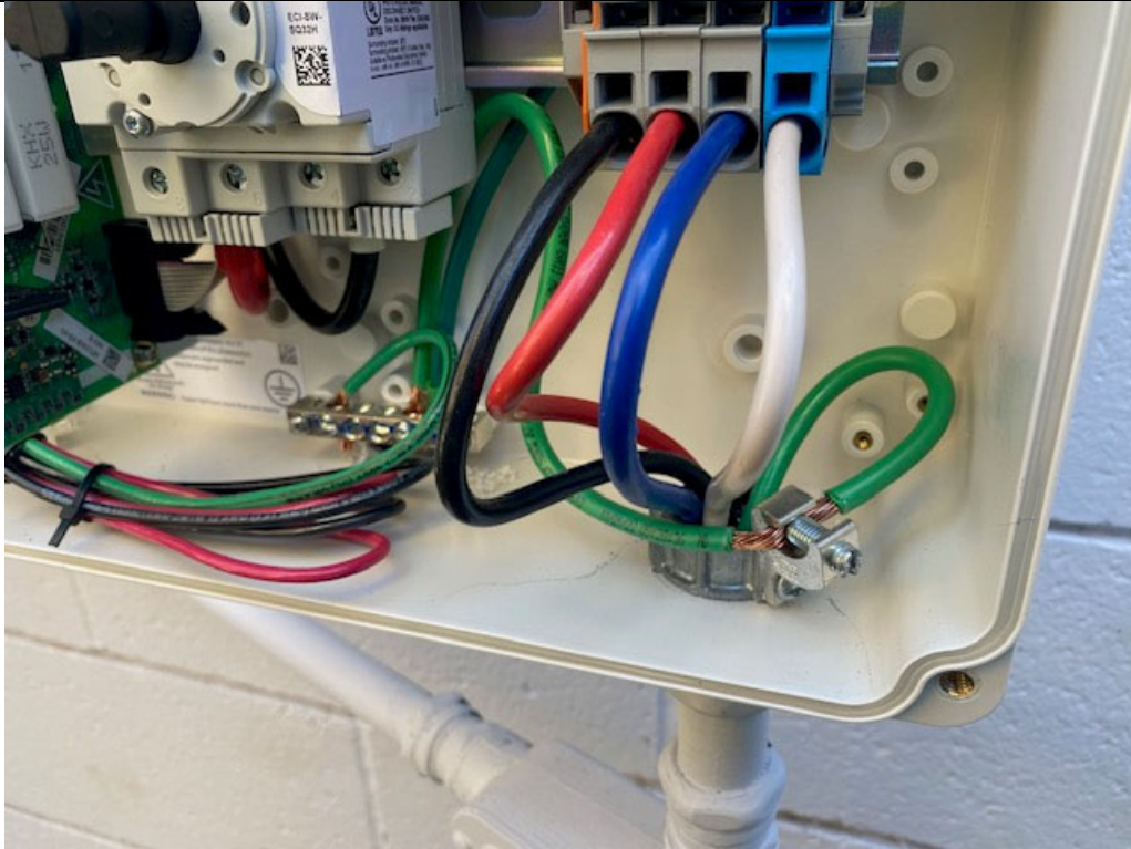
Photo 3 – EMT Into Non-metallic Enclosure
