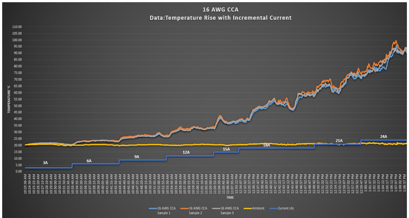
Graph 1: 16 AWG CCA
