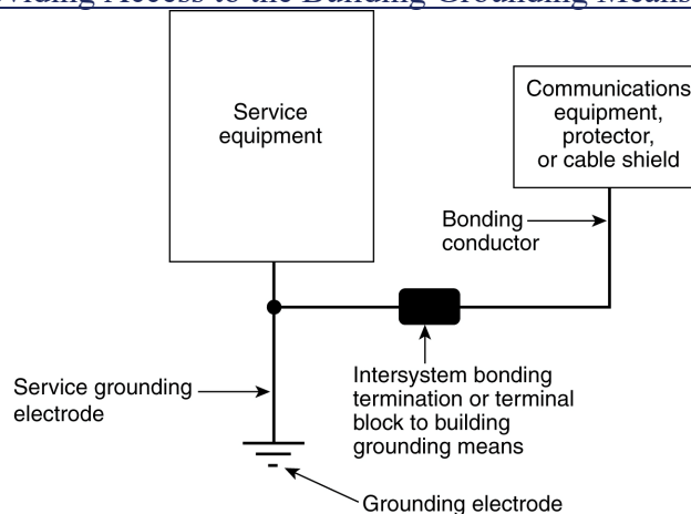
Figure Informational Note 251.100(B)(1) Illustration of a Bonding Conductor in a Communications Installation Equipped with an Intersystem Bonding Termination or Terminal Block Providing Access to the Building Grounding Means.
