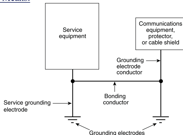
Figure Informational Note 251.100(B)(2) Illustration of a Grounding Electrode Conductor and a Bonding Conductor in a Communications Installation Not Equipped with an Intersystem Bonding Termination or Terminal Block Providing Access to the Building Grounding Means.
