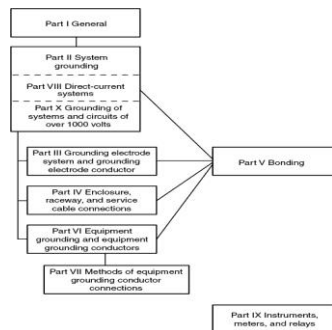
Figure Informational Note Figure 350.1 Grounding and Bonding.
