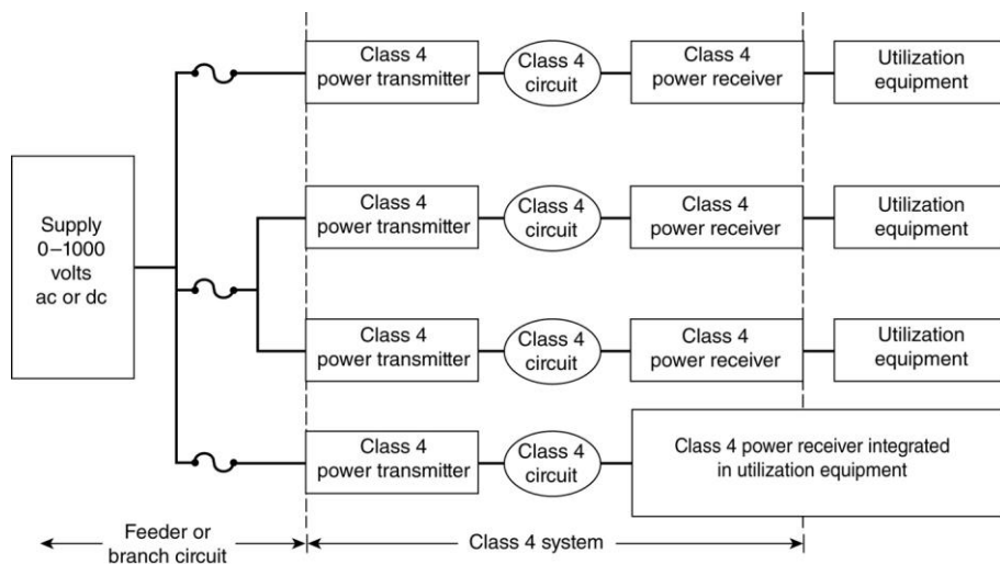
Informational Note Figure 726.124-792.50 Class 4 Circuits.
