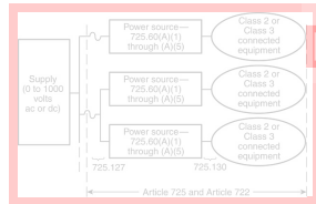
Figure Informational Note 792.30 Class 2 and Class 3 Circuits.
