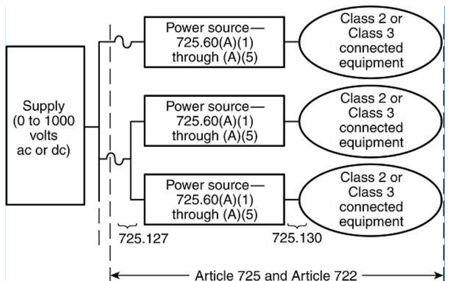
Informational Note Figure 792.30725-60 Class 2 and Class 3 Circuits.
