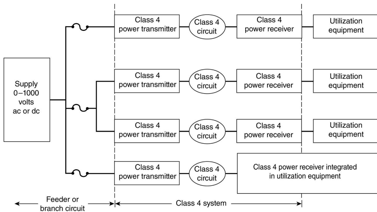
Figure Informational Note Figure 726.121 Class 4 Circuits.
