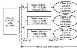
Figure Informational Note 792.30(A) Class 2 and Class 3 Circuits.
