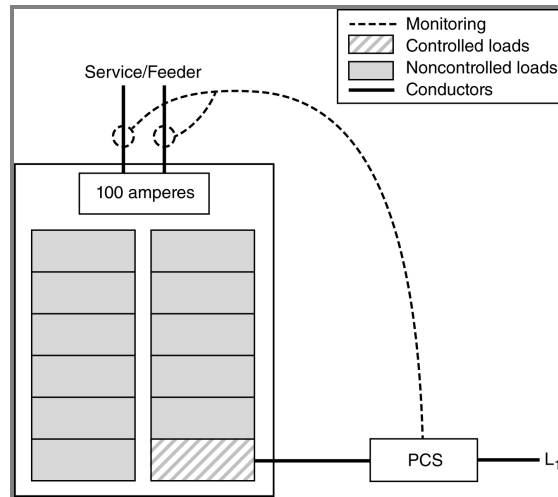
Figure D.15(b) Monitoring Controlled and Noncontrolled Loads, 30-Ampere EVSE.
