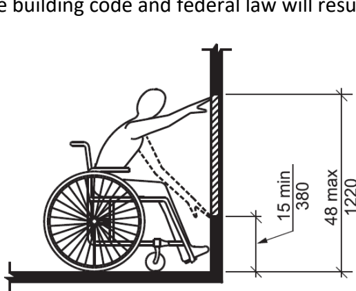
FIGURE 308.2.1 UNOBSTRUCTED FORWARD REACH
