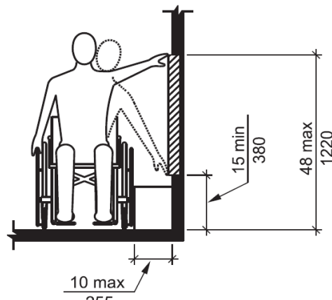
FIGURE 308.3.1 UNOBSTRUCTED SIDE REACH
