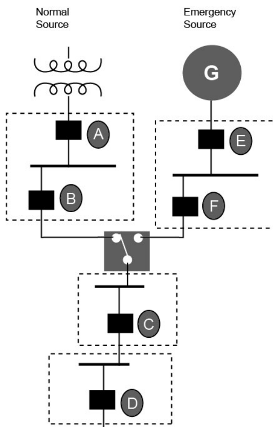
Figure Informational Note Figure 700.32 Emergency System Selective Coordination.
