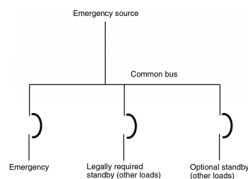
Figure Informational Note Figure 700.10(B)(b) Single or Multiple Feeders with Overcurrent Protection.
