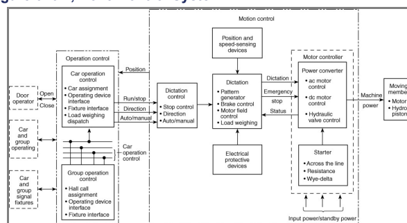
Figure Informational Note Figure 620.1, No. 5 Control System.
