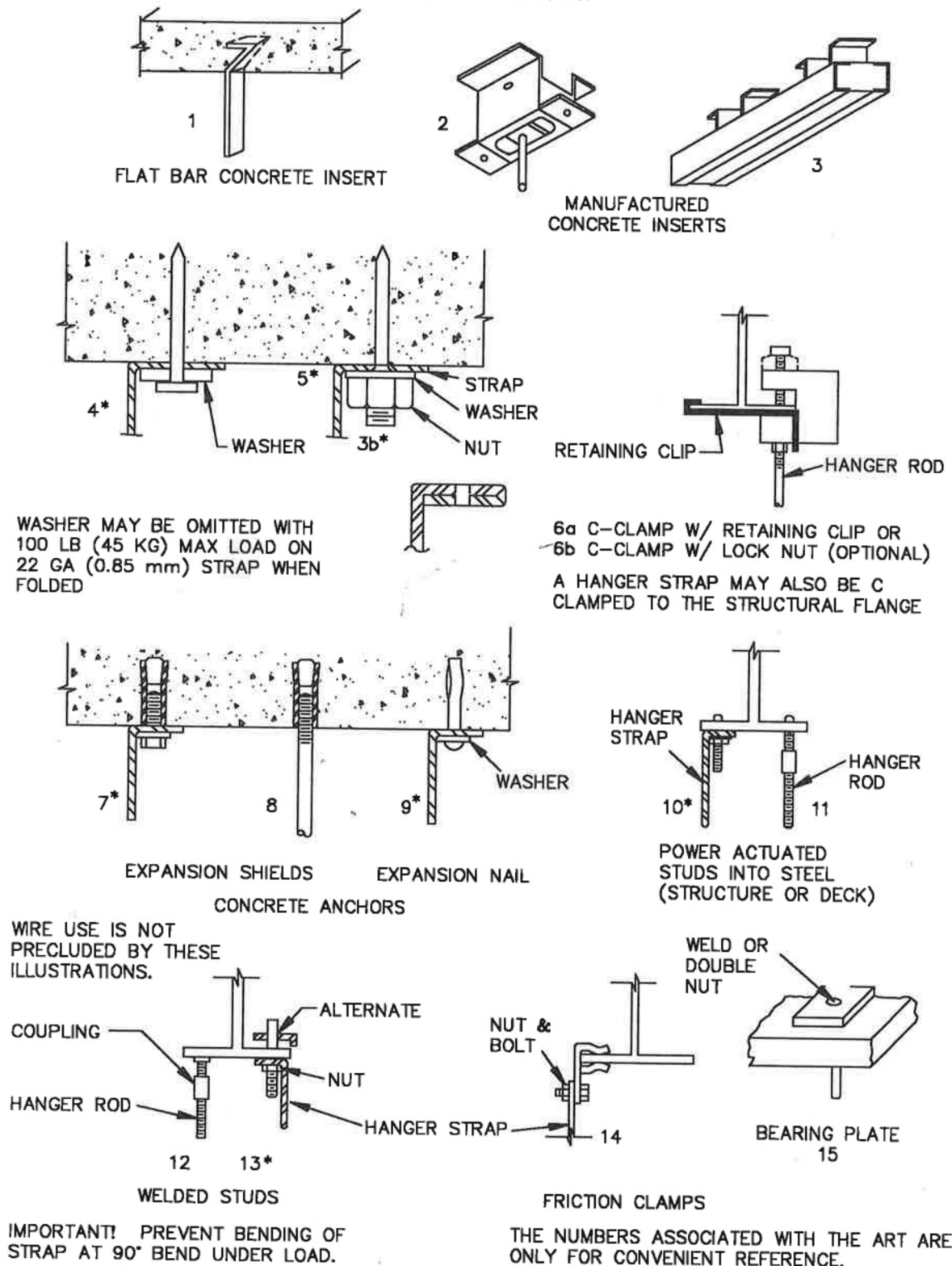
UPPER ATTACHMENT DEVICES - TYPICAL
