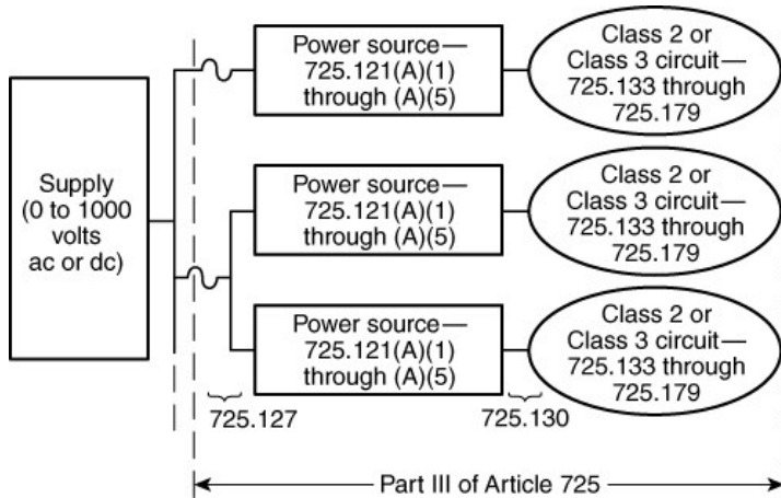
Informational Note Figure 725.121 Class 2 and Class 3 Circuits.
