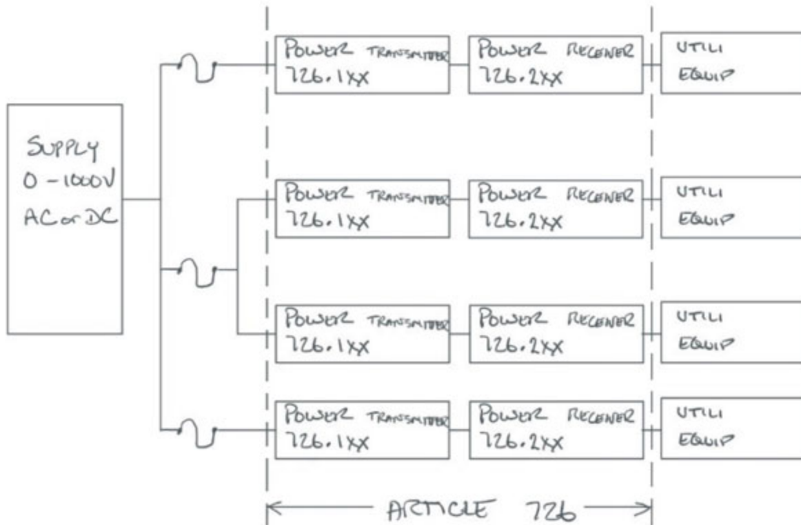
Informational Note No. 1 Figure 726.121 Class 4 Circuits
