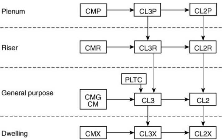
Figure 725.154(A) Cable Substitution Hierarchy.
