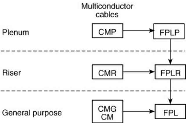
Figure 760.154(A) Cable Substitution Hierarchy.
