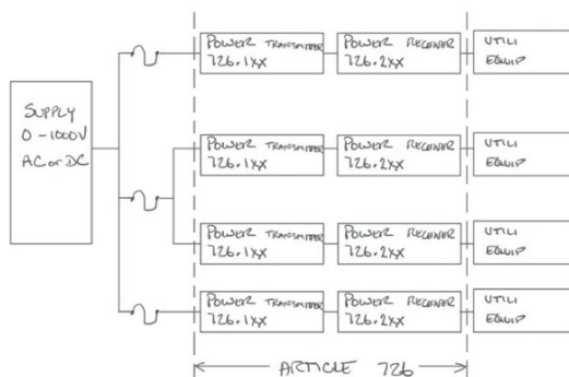
Informational Note No. 1 Figure 726.121 Class 4 Circuits
