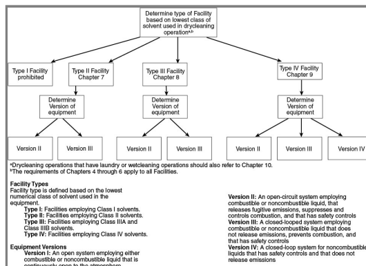
Figure B.1 NFPA 32 Document Requirements Flowchart.
