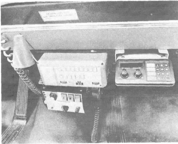
Figure 4-6(k) Left: 4-frequency mobile radio control head with electronic siren/public address system below. Right: 20-frequency programmable scanner as mounted in sedan.
