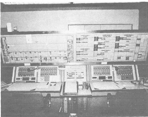
Figure 5-6(e) Two-position dispatch and communications console with resource directories, tone encoder, tape recorder, and resource/situation display.
