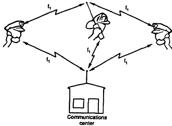
Figure 4-4 Single-frequency simplex operation.
