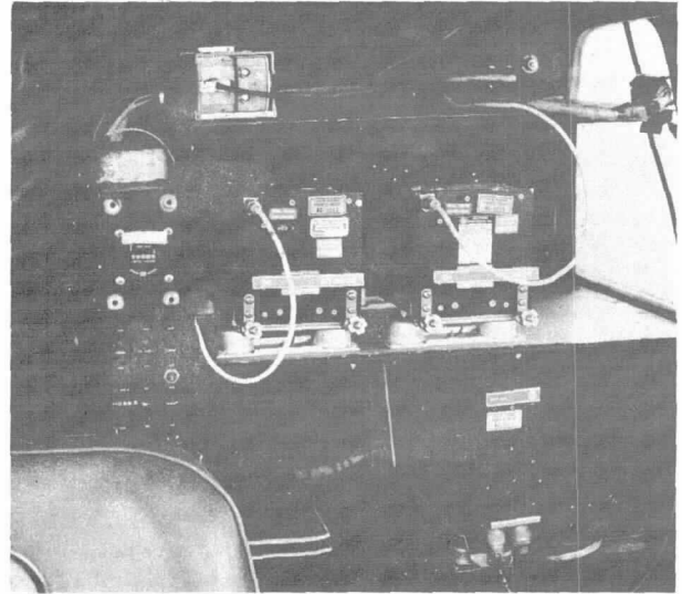
Figure 4-6(d) 9600-channel air-to-air and air-to-ground radios as installed in light observation air attack aircraft.
