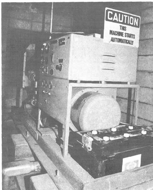
Figure 4-6(g) . Emergency standby electric power generator.
