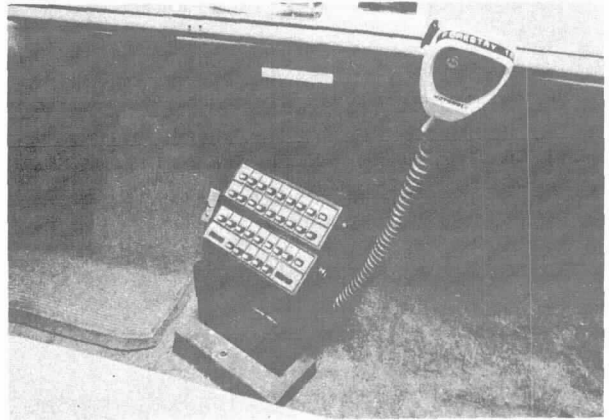
Figure 4-6(e) 32-channel synthesized mobile transmitter-receiver unit. Mobile unit also includes an 8-channel scanner with two levels of priority and is capable of 16 tones on any of the 32 transmit frequencies.
