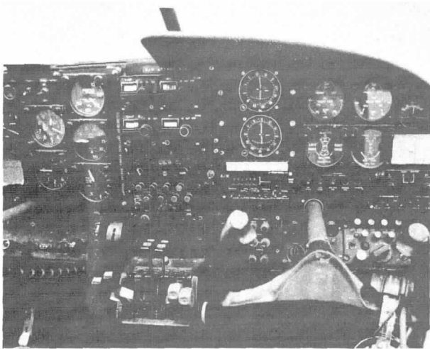
Figure 4-6(c) Air-to-air and air-to-ground control heads as installed in light observation/air attack aircraft (to left and right of right-hand control). Note mixer box for various aircraft radios in lower right.
