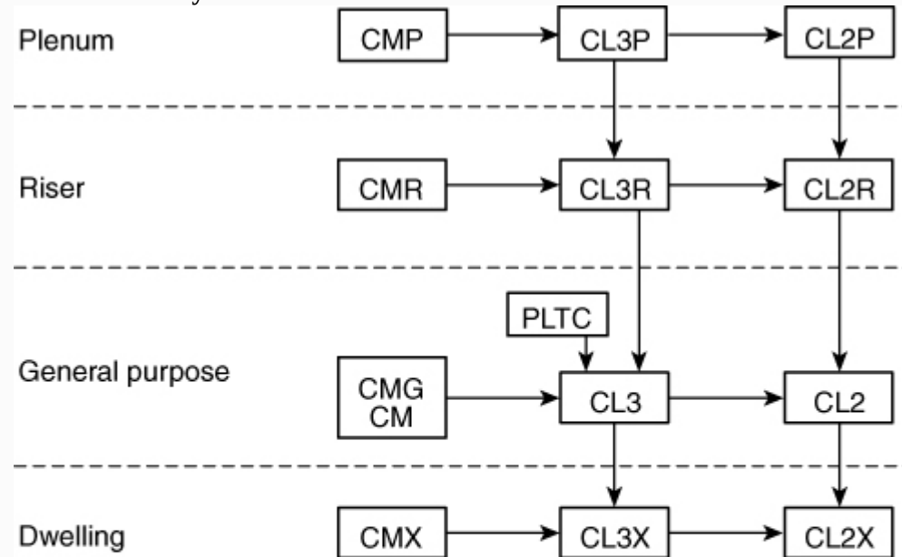
Figure 725.154(A) Cable Substitution Hierarchy.
