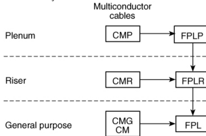
Figure 760.154(A) Cable Substitution Hierarchy.
