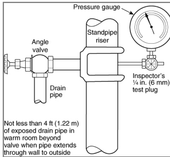
Figure 7.11.2.1 Drain Connection for System Riser.
