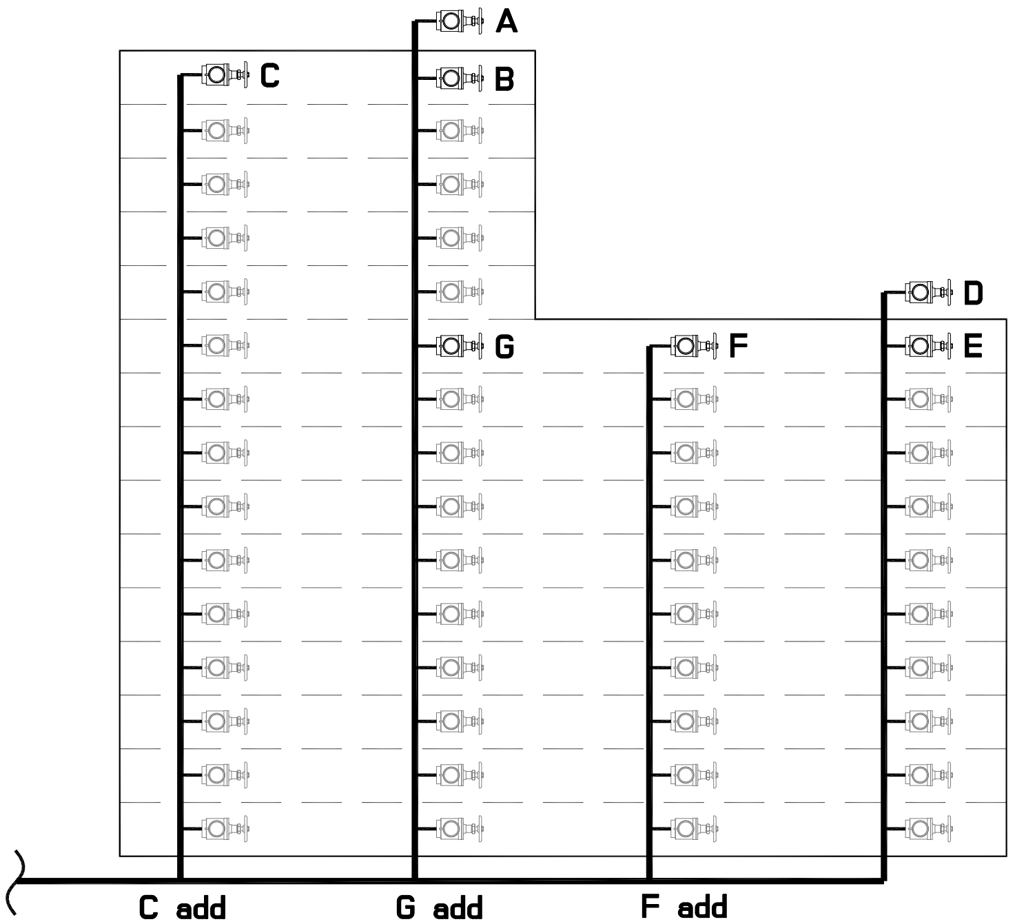
Figure A.7.10.1.2.1 Standpipe System with Risers Terminating at Different Floor Levels
