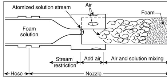
Figure 5.3.1.2.1(b) Combination Nozzle with Low-Expansion Foam Attachment.
