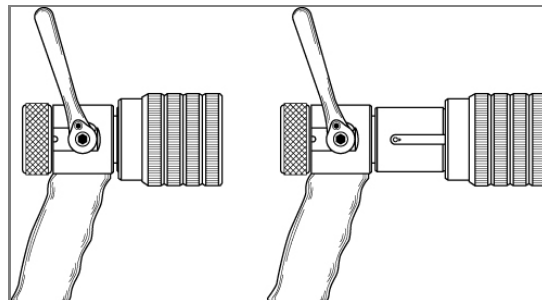
Figure 5.3.1.2.1(e) Combination Nozzle with Retractable Sleeve.
