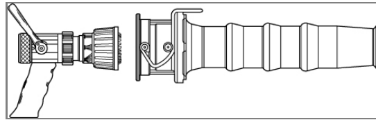
Figure 5.3.1.2.1(c) Combination Nozzle with Multi-Expansion Foam Attachment.
