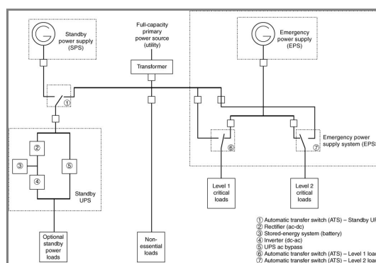
Figure B.1(d) Simplified Diagram for an Emergency Power Supply System (EPSS) and a Standby UPS.
