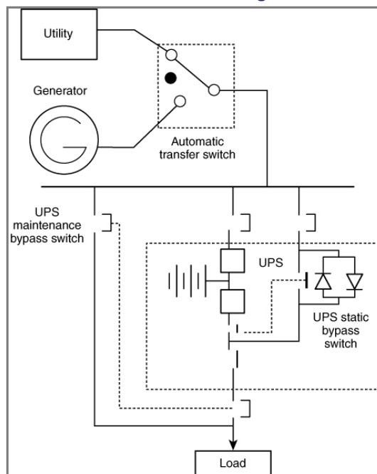
Figure A.6.1.1 Simplified One-Line SEPSS Switching Points.
