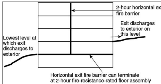
Figure A.7.2.4.3.2 Example of Horizontal Exit Termination.
