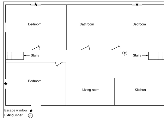
Figure A.24.6.2.1 Short-Term Rental Unit Floor Sample Diagram.
