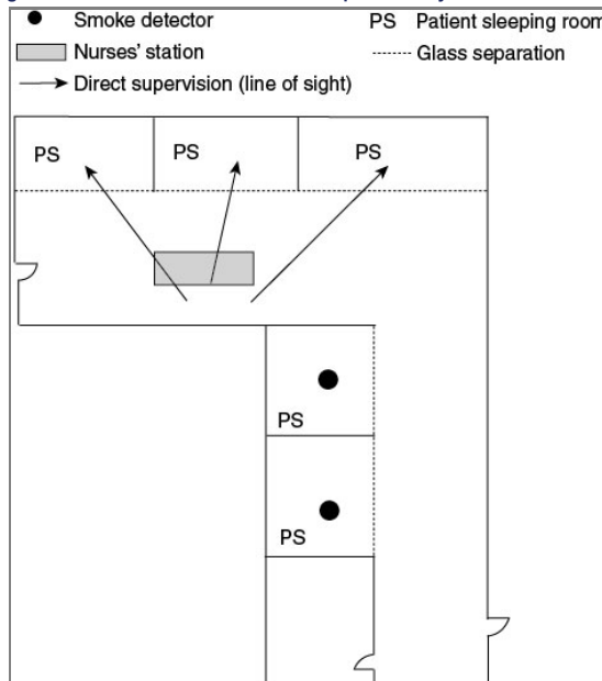
Figure A.18.2.5.7.2.1(B) All Sleeping Rooms Provided with Either Direct Supervision by Staff or Smoke Detection.
