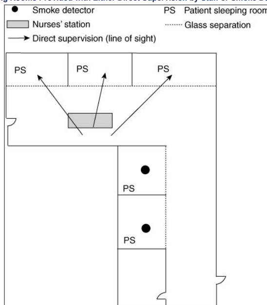
Figure A.19.2.5.7.2.1(B) All Sleeping Rooms Provided with Either Direct Supervision by Staff or Smoke Detection.
