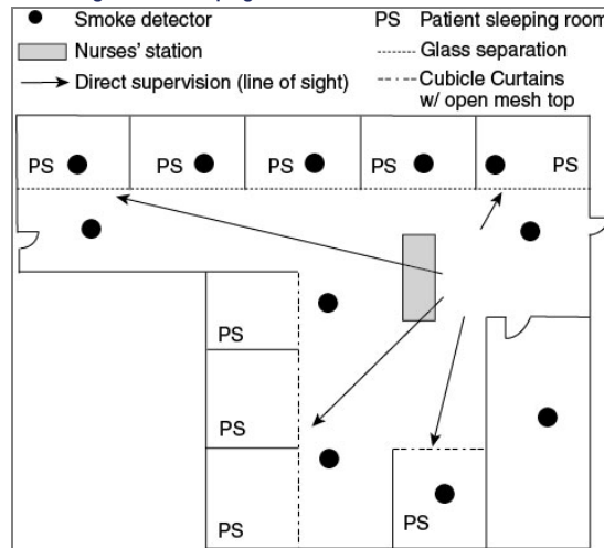
Figure A.18.2.5.7.2.3(C) For Suites >7500 ft 2 (>700 m 2 ), All Sleeping Rooms Must Be Provided with Direct Supervision by Staff and Total (Complete) Smoke Detection Installed Throughout the Sleeping Suite.
