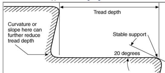
Figure A.7.2.2.3.5(e) Tread Measurement with Unstable Stepping Surface at Leading Edge.
