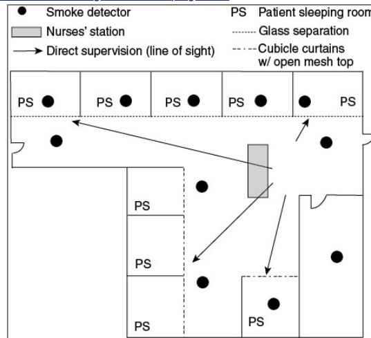
Figure A.19.2.5.7.2.3(C) For Suites >7500 ft 2 (>700 m 2 ). All Sleeping Rooms Must Be Provided with Direct Supervision by Staff and Total (Complete) Smoke Detection Installed Throughout the Sleeping Suite.
