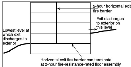
Figure A.7.2.4.3.2 Example of Horizontal Exit Termination.
