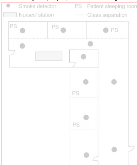
Figure A.19.2.5.7.2.1(B)(c) For Suites >5000 ft 2 (>460 m 2 ) and ≤7500 ft 2 (≤700 m 2 ) Protected by Standard Response Sprinklers, Total (Complete) Smoke Detection Required Throughout the Sleeping Suite.
