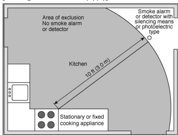
Figure A.9.6.2.10.5(a) Example of Zone of Exclusion (gray area) Within Typical Residential Kitchen. [72: Figure A.29.8.3.4(4)(a)]
