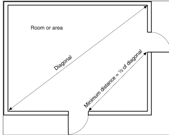
Figure A.7.5.1.3.2(b) Diagonal Rule for Exit and Exit Access Door Remoteness.
