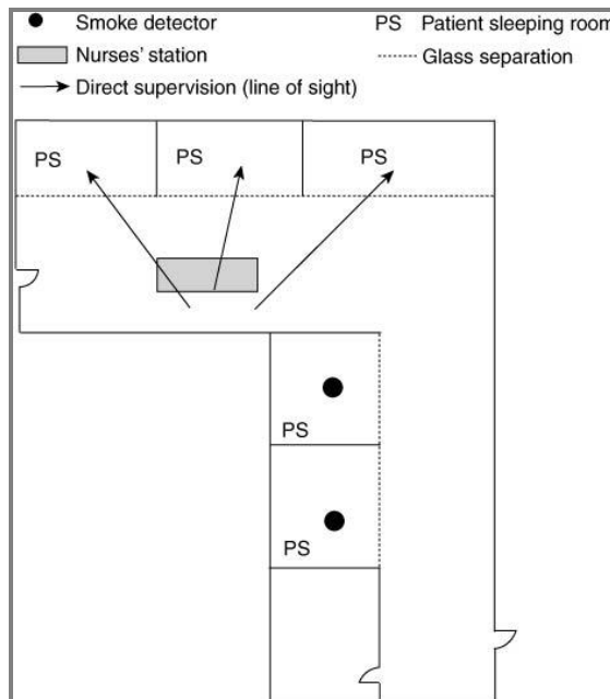
Figure A.19.2.5.7.2.1(B) All Sleeping Rooms Provided with Either with Direct Supervision by Staff or Smoke Detection.
