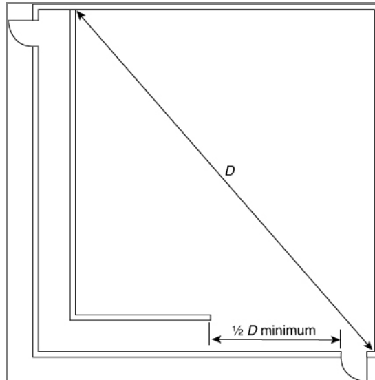
Figure A.7.5.1.3.2(d) Exit Separation and Diagonal Measurement of Area Served.
