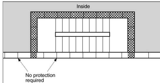
Figure A.7.2.2.5.2(b) Stairway with Unprotected Exterior Perimeter Protruding Past Building Exterior Wall.
