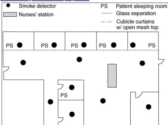
Figure A.19.2.5.7.2.3(B) For Suites >5000 \text{ ft}^2 ( >460 \text{ m}^2 ) and \leq 7500 \text{ ft}^2 ( \leq 700 \text{ m}^2 ) Protected by Standard Response Sprinklers, Total (Complete) Smoke Detection Required Throughout the Sleeping Suite.
