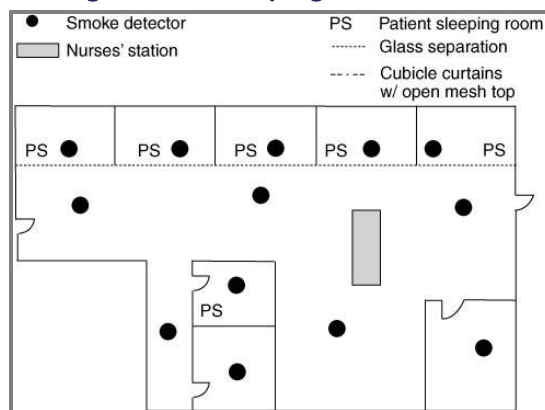
Figure A.19.2.5.7.2.3(B) For Suites >5000 ft 2 (>460 m 2 ) and ≤7500 ft 2 (≤700 m 2 ) Protected by Standard Response Sprinklers, Total (Complete) Smoke Detection Required Throughout the Sleeping Suite.
