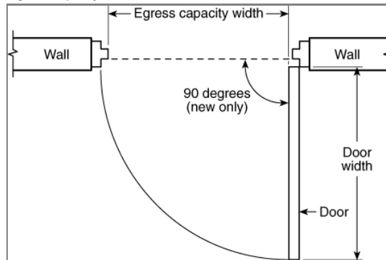
Figure A.7.2.1.2.2(b) Door Width — Egress Capacity with Permitted Obstructions.
