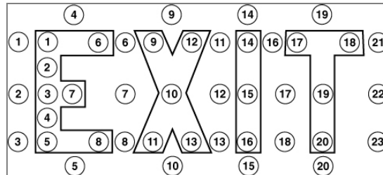
Figure A.7.10.6.3 Measurement of Exit Sign Luminance.
