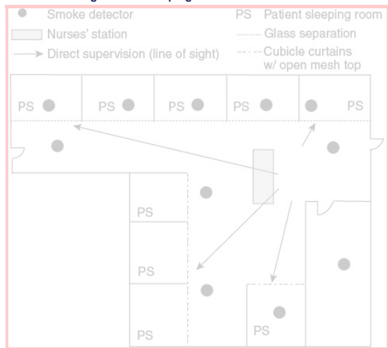
Figure A.19.2.5.7.2.1(B)(d) For Suites >7500 \text{ ft}^2 ( >700 \text{ m}^2 ), All Sleeping Rooms Must Be Provided with Direct Supervision by Staff and Total (Complete) Smoke Detection Installed Throughout the Sleeping Suite.
