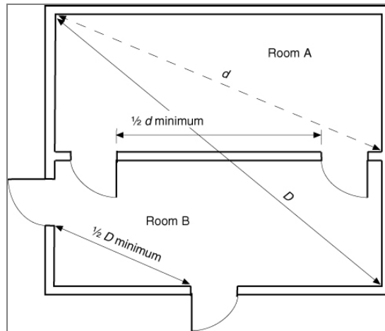
Figure A.7.5.1.3.2(c) Diagonal Rule for Exit and Access Remoteness.
