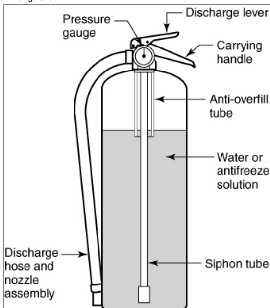
Figure D.4.1.1 Stored-Pressure Water Extinguisher.
