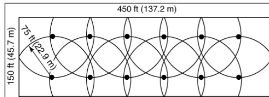
Figure E.3.12 Configuration Representing 12 Fire Extinguishers Mounted on Building Columns in Which Requirements for Both Travel Distance and Fire Extinguisher Distribution Are Met.
