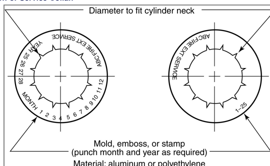
Figure A.7.13 Design of a Verification-of-Service Collar.
