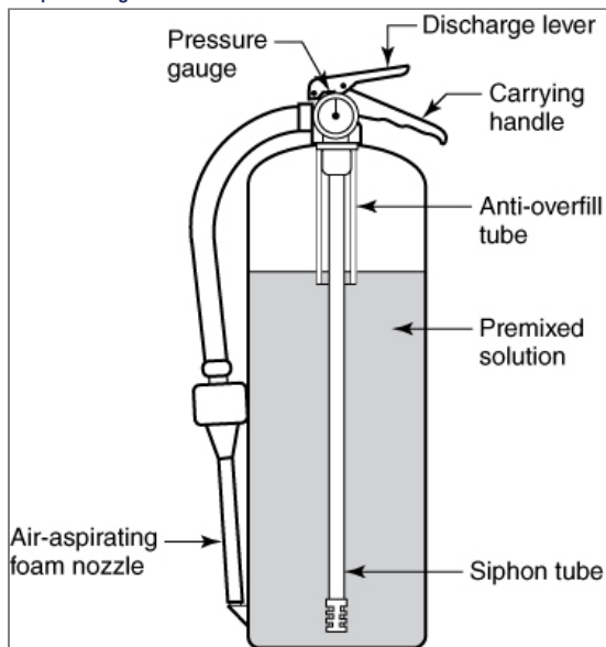
Figure D.4.2.1 Stored-Pressure Foam Liquid Extinguisher.
