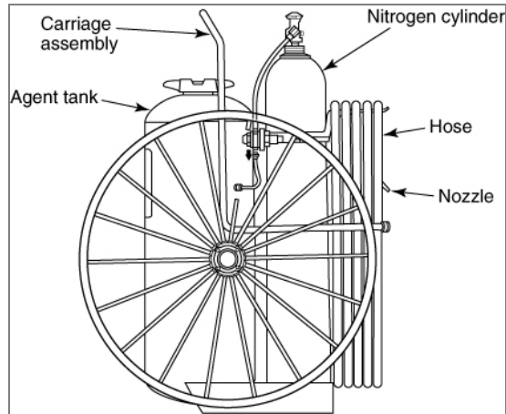
Figure C.3.7.2(b) Stored-Pressure Halogenated Agent Type.
